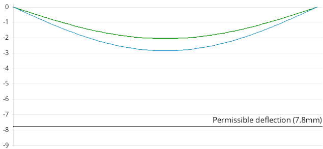
Live load deflection (green) and total load deflection (blue) in mm
